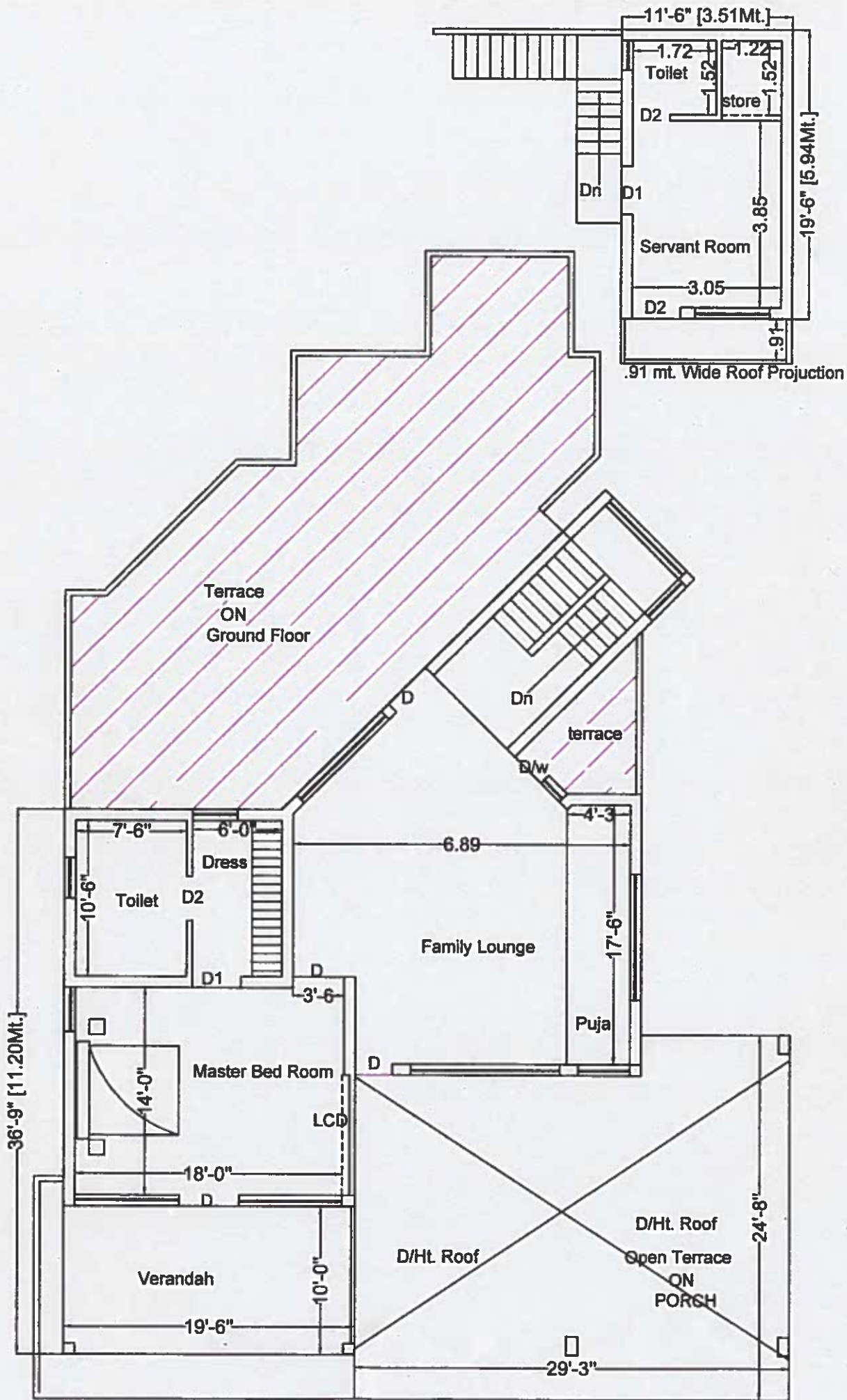
First Floor Area (107.88 m2)
